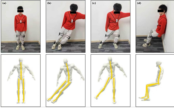
Fig. 3. Representative static posture cases and corresponding UI snapshots. The top row shows the four tested static postures: (a) neutral standing, (b) parallel edging stance, (c) A-frame posture, and (d) backseat posture. The bottom row shows the corresponding UI outputs of the proposed posture monitoring system.
