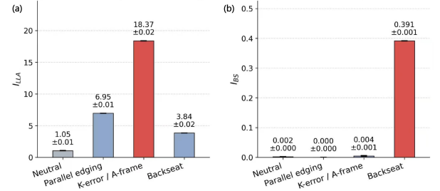
Fig. 4. Static posture indicator responses under four representative static postures. (a) Lower-limb alignment indicator I_{LLA} . (b) Backseat tendency indicator I_{BS} . Error bars and text labels indicate the 95% confidence interval half-width estimated from the selected stable segment.
